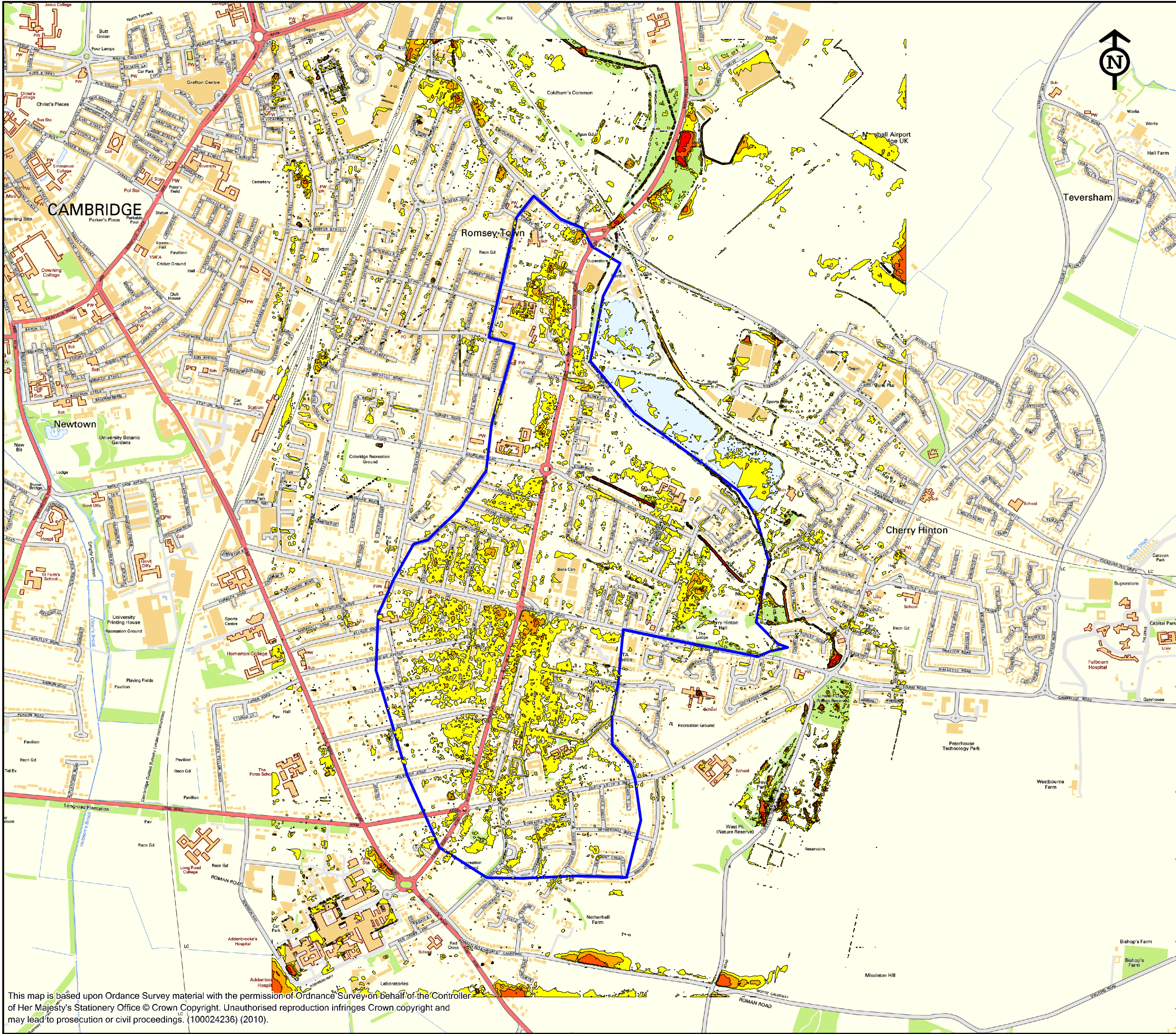
FIGURE G22 1.33% AEP "DO NOTHING" PLUVIAL MODELLING MAXIMUM DEPTH CHERRY HINTON
